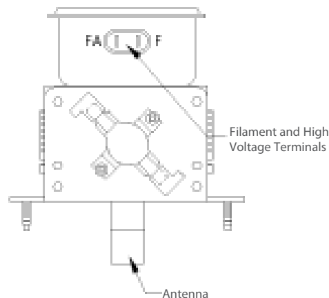
Figure 41: Magnetron Detail
