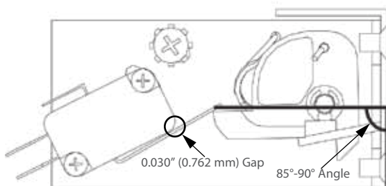
Figure 38: Switch Detail and Proper Alignment
