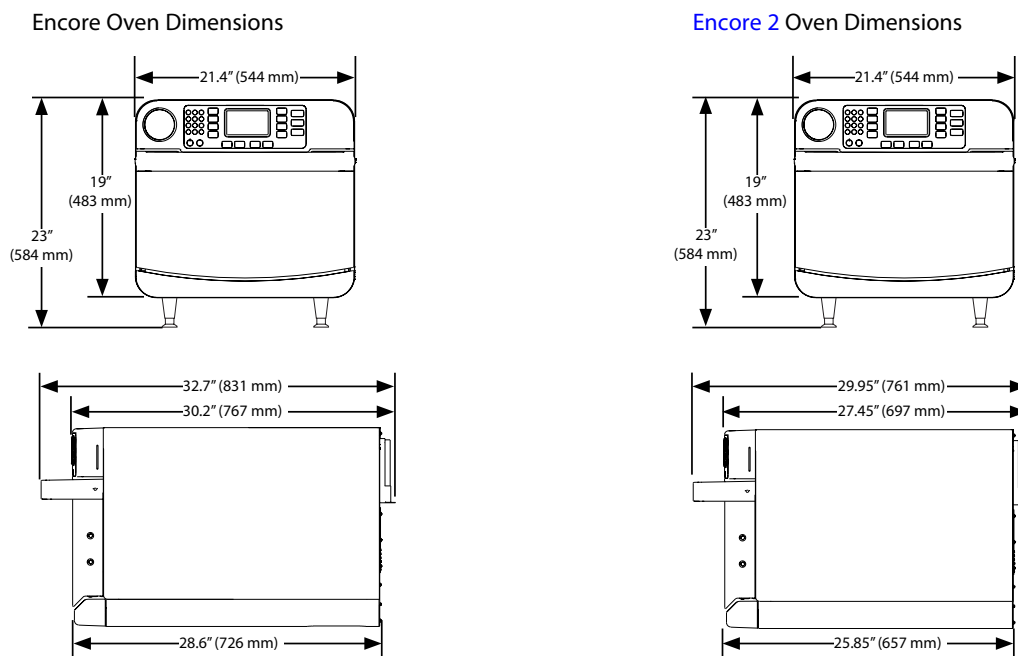
Figure 1: Encore and Encore 2 Oven Dimensions
