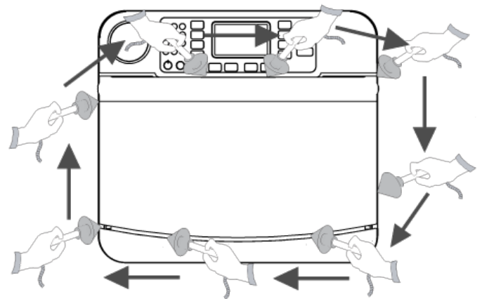
Figure 39: Measure for Microwave Leakage
